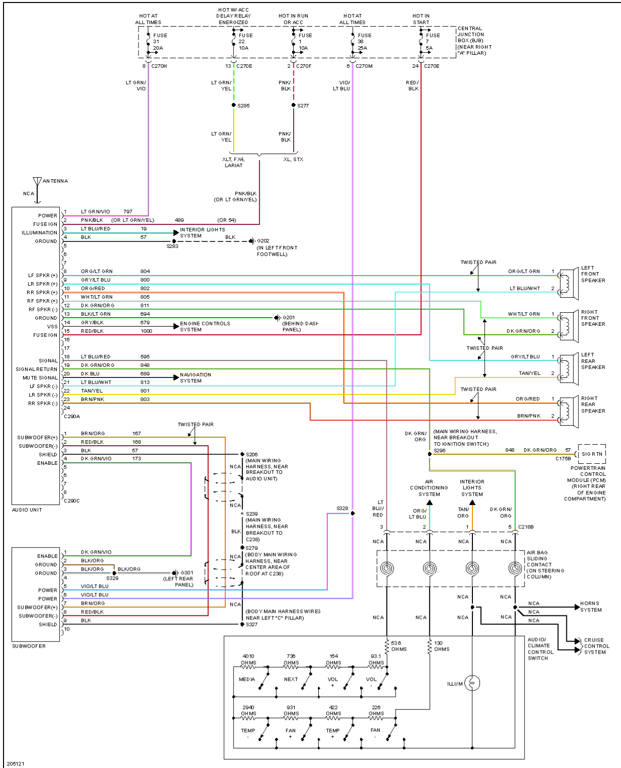
Fig. 70: Premium Sound Radio Circuit, W/O DVD
