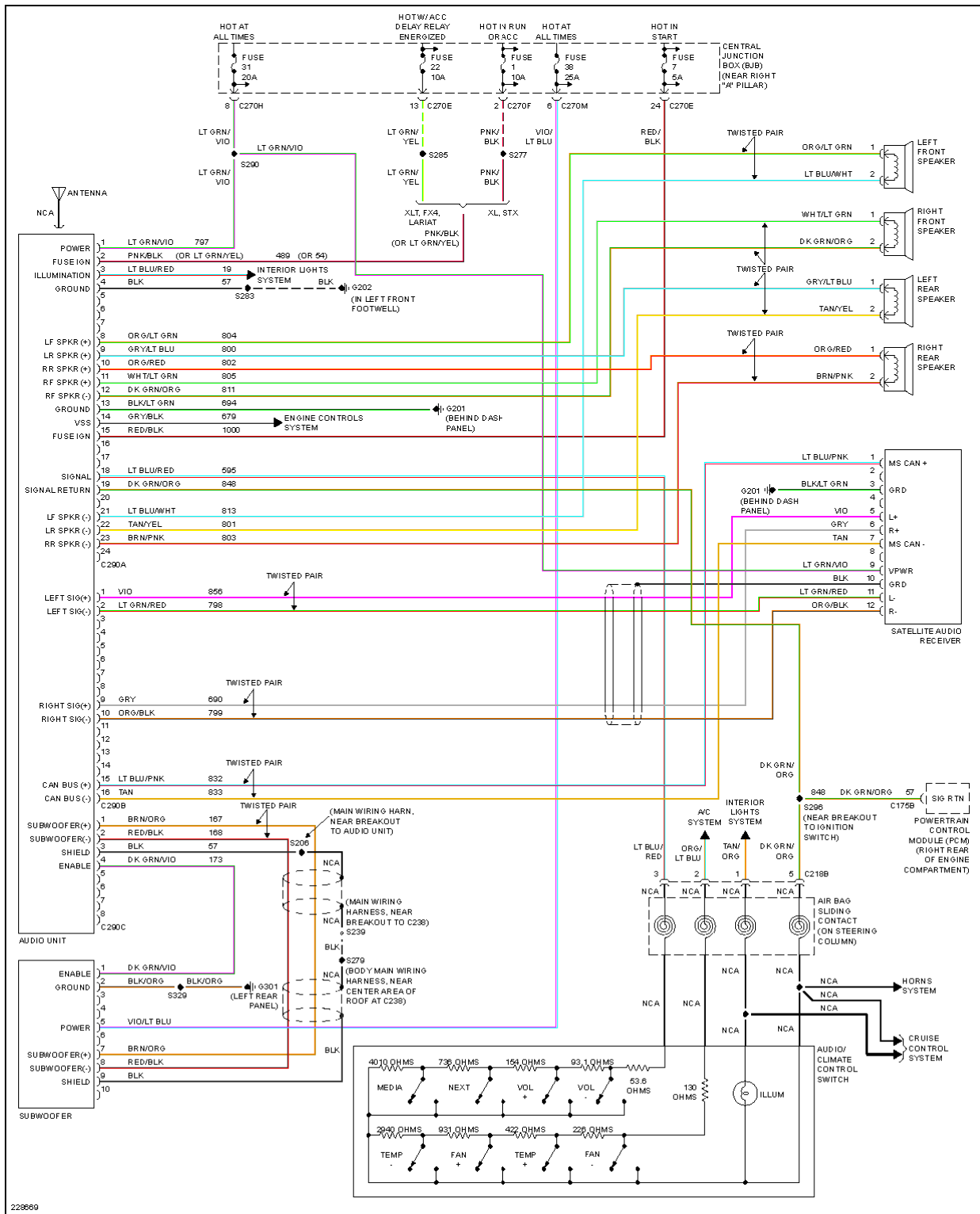
Fig. 69: Premium Sound Radio Circuit, W/ Satellite Radio
